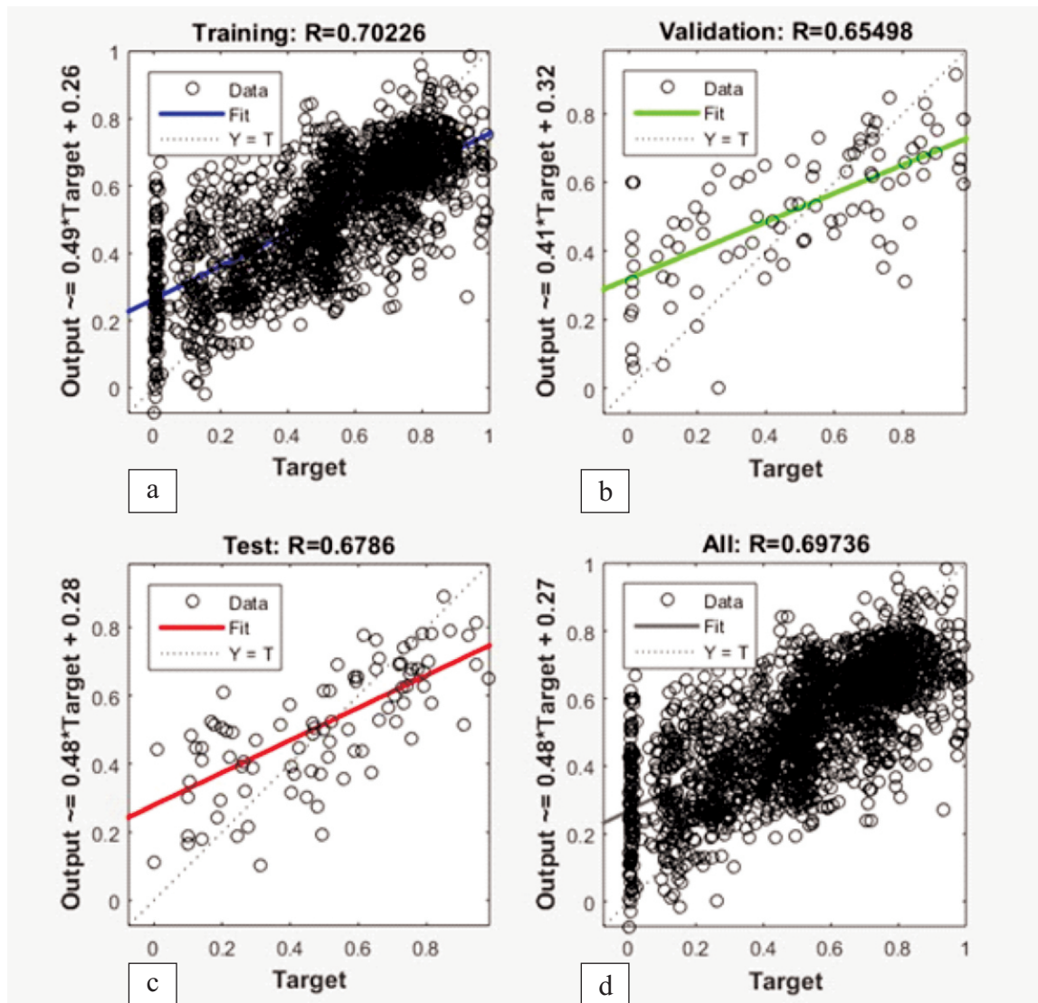
Figure VI: Regression plots
