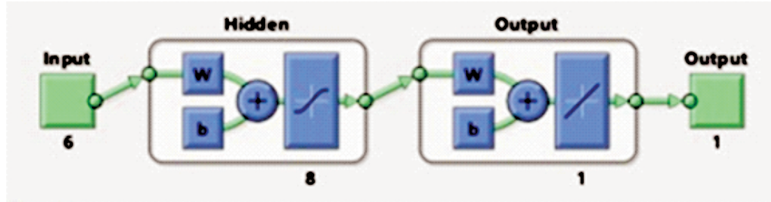
Figure IV: FFNN Model
