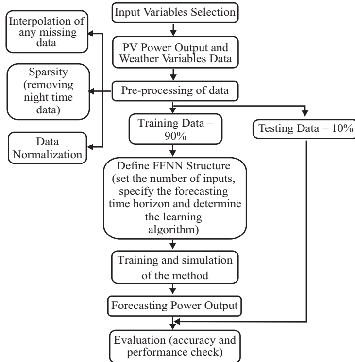
Figure II: Flowchart for the proposed PV power forecasting technique
