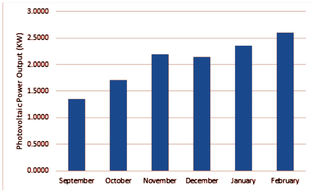
Figure V: Monthly total DC power produced from September 2021 to February 2022.
