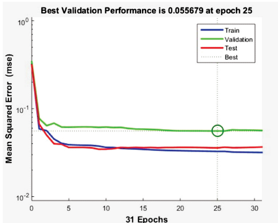
Figure VII: Performance Plot
